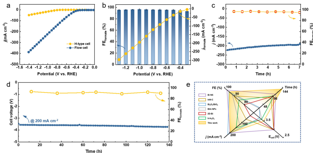
Fig. 3 High-throughput CO 2 RR performance. (a) LSV curves of Bi 5 O 7 I NTs in the H-type cell and flow cell, (b) FE formate and j_{\text{formate}} of Bi 5 O 7 I NTs at all potentials in the flow cell, (c) stability test of Bi 5 O 7 I NTs at -1.0 V vs. RHE in the flow cell, (d) the CO 2 RR performance of Bi 5 O 7 I NTs at 200 mA cm -2 in the MEA system, and (e) comparison of the FE formate , j , E_{\text{cell}} and stability of recently reported electrocatalysts for the CO 2 RR to formate in the MEA system.
