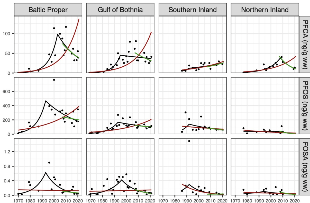
Fig. 3 Change-point graphs for the summed concentration of PFCA, PFOS and FOSA across the four sampling regions. Each dot represents a yearly geometric average. Change-point trends are provided in black, while log-linear trends for the whole period and last 15 years are shown in red and green, respectively. Statistical significance is provided in Table 1.
