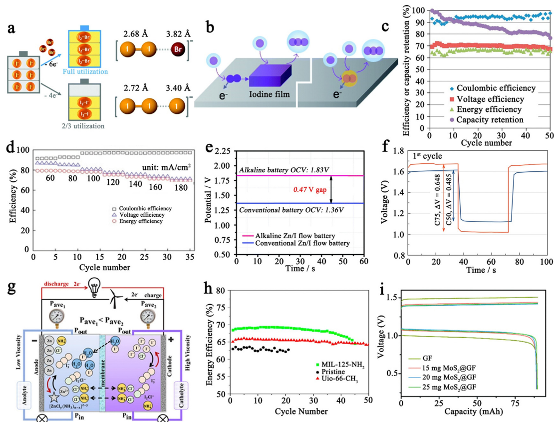
Fig. 17 (a) Schematic representation of Br - ions as complexing agents for iodine stabilization. Reprinted with permission from ref. 227. Copyright 2017 Royal Society of Chemistry. (b) The working mechanisms of I - to I 3 - transition without (left) and with (right) a cosolvent in an aqueous solution. Reprinted with permission from ref. 228. Copyright 2022 Royal Society of Chemistry. (c) Efficiencies of ZIRFB at 20 mA cm -2 with the electrolyte of 1.5 M NaI, 0.5 M ZnCl 2 , 1.0 vol% PEG200 (polyethyleneglycoland), and 0.15 vol% HCl with 20 vol% propylene carbonate. Reprinted with permission from ref. 229. Copyright 2019 Elsevier. (d) Rate capability of ZIRFB with an electrolyte of 2 M KI + 1 M ZnBr 2 . Reprinted with permission from ref. 231. Copyright 2018 Wiley. (e) Open-circuit voltage of conventional and designed alkaline ZIRFBs. Reprinted with permission from ref. 164. Copyright 2018 Royal Society of Chemistry. (f) Polarization voltage curves for C50 (CMC : PVA = 50 : 50 wt%) and C75 (CMC : PVA = 75 : 25 wt%) cells show decent performance and cycling stability at 10 mA cm -2 for the first cycle. Reprinted with permission from ref. 220. Copyright 2022 Elsevier. (g) Schematic diagram of ion convection caused by unbalanced hydraulic pressure in a ZIRFB. Reprinted with permission from ref. 237. Copyright 2021 Elsevier. (h) Cycling performance of ZIRFBs with the pristine graphite felt and the MOF-modified graphite felt electrodes. Reprinted with permission from ref. 239. Copyright 2016 American Chemical Society. (i) Charge-discharge curves of the pristine graphite felt, and the MoS 2 -modified graphite felt electrodes at 30 mA cm -2 . Reprinted with permission from ref. 238. Copyright 2019 Royal Society of Chemistry.
