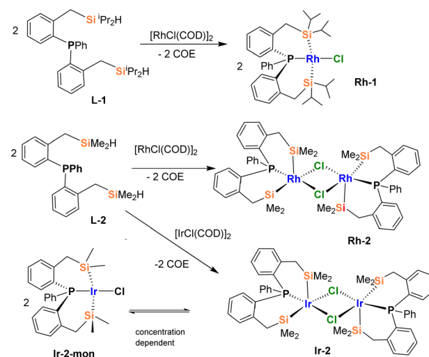
Scheme 1 The synthesis of Rh and Ir(III) complexes bearing methyl or isopropyl substituted ( \kappa^3\text{-Si,Si,P} ) silylphosphine ligands.
