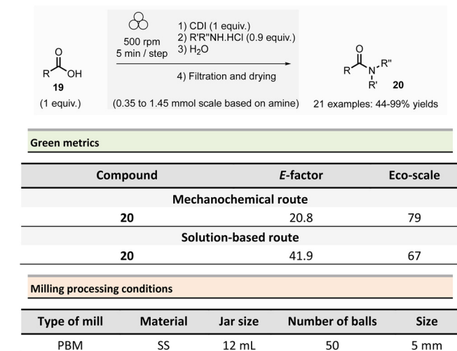
Scheme 5 CDI-mediated amidation by mechanochemistry.
