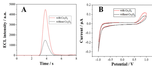
Fig. 1 (A) ECL profiles and (B) CV curves of the L12- \text{H}_2\text{O}_2 system at the ITO surface with and without \text{Co}_3\text{O}_4 . Working solution: 10 mM PBS containing 200 \mu\text{M} L12. Scan range: -1.0 to 1.0 V, scan rate: 0.1 V \text{s}^{-1} , PMT voltage: 600 V.
