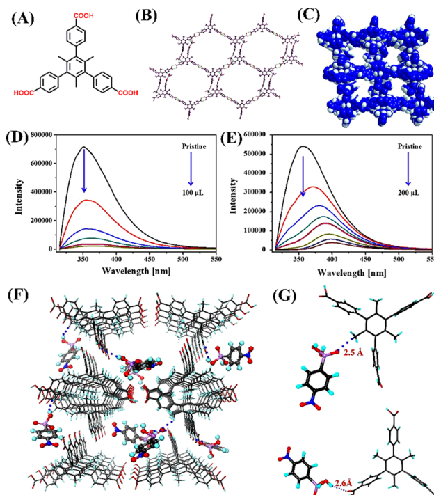
Fig. 11 (A) The structures of ligand H 3 CTTA; (B) crystal structure of HOF-22 showing a 2D layer formation from adjacent chains; (C) representation of HOF-22 porous framework; the observed relative changes in fluorescence emission intensity for HOF-22 after adding (D) p -NIT and (E) ROX; (F) the simulated structure of p -NIT loaded HOF-22 and (G) selected fragments indicating the hydrogen-bonding interactions between HOF-22 and p -NIT. Reprinted with permission from ref. 87. Copyright 2020 Canadian Science Publishing.
