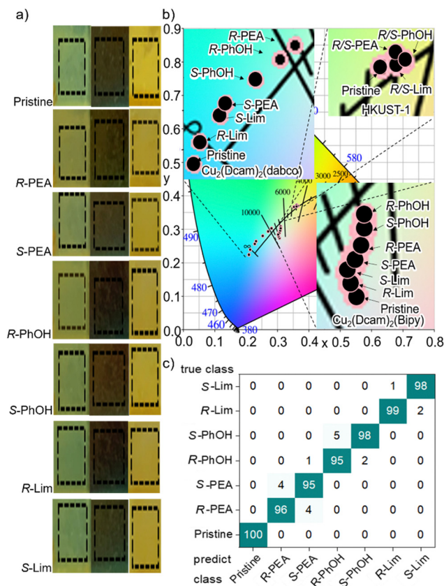
Fig. 4 (a) The FP-SURMOF sensors (left: \text{Cu}_2(\text{DCam})_2(\text{dabco}) , center: \text{Cu}_2(\text{DCam})_2(\text{Bipy}) and right: HKUST-1) in an atmosphere of the different analytes, see labels. The dotted squares are the areas where the color (i.e. the RGB values, see Table S1, ESI†) were determined. (b) The sensors on the CIE-color-space map. (c) The confusion matrix to classify the chiral odors, calculated by ANN.
