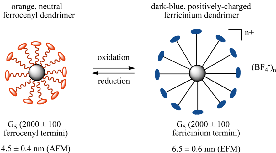
Fig. 8 Redox breathing of a 5th generation ferrocenyl-terminated dendrimer constructed according to Scheme 6 followed by the reaction of G_5 -CH 2 I with \text{Fc}(\text{CH}_2)_{11}\text{O}-p\text{-C}_6\text{H}_4\text{OH} in the presence of \text{K}_2\text{CO}_3 in DMF for 2 d at 80 °C. 87
