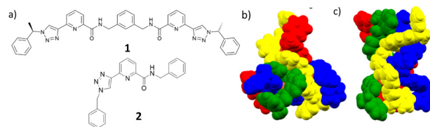
Fig. 1 (a) The chiral bis-tridentate (1,2,3-triazol-4-yl)-picolinamide (tzpa) ligand 1 used in the current study, and the ‘half’ ligand 2, which was formed as a model ligand. The solid state structures of the tetranuclear [2 × 2] square grids formed from 1 in our previous study using: (b) Cu(NO 3 ) 2 ·3 H 2 O and (c) [Cu(MeCN) 4 ](PF 6 ), respectively. 26
