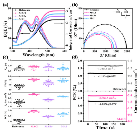
Fig. 3 (a) The EQE and integrated current density curves of the PSCs. (b) Nyquist EIS spectra (the inset is the equivalent circuit). (c) Box charts of V_{oc} , FF, J_{sc} and PCE. (d) Steady-state power outputs at the maximum power point of the reference and Cs 2 AgBiBr 6 -MACl.
