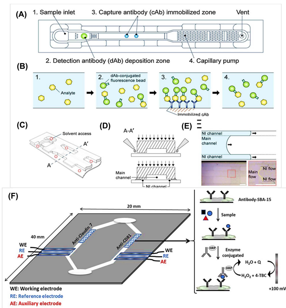
Fig. 3 Microfluidic immunoassay. Schematic illustration of (A) the microfluidic device comprising immunoassay elements and (B) interactions between antibodies and analytes along the sample flow. (C) Structure showing solvent access for the assembled device. (D) Cross-sectional view of the nanointerstice (NI) channel generated by solvent bonding (A–A'). (E) The air–liquid interface (ALI) in the channel filling flow. Reproduced with permission from Kim et al. , Sens. Actuators B Chem. , 2020, 316 , 128094. Copyright 2020, Elsevier. (F) Schematic representation of the electrochemical paper-based immunosensor for Claudin 7 and CD81 dual determination. Reproduced with permission from Ortega et al. , Anal. Chem. , 2021, 93 , 1143–1153. Copyright 2021, American Chemical Society.
