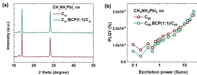
Fig. 5 (a) X-Ray diffraction patterns of \text{CH}_3\text{NH}_3\text{PbI}_3 films grown on \text{ITO}/\text{C}_{60} and \text{ITO}/\text{C}_{60}:\text{BCP}/\text{C}_{60} and (b) photoluminescence quantum yield (PLQY) under different excitation powers.
