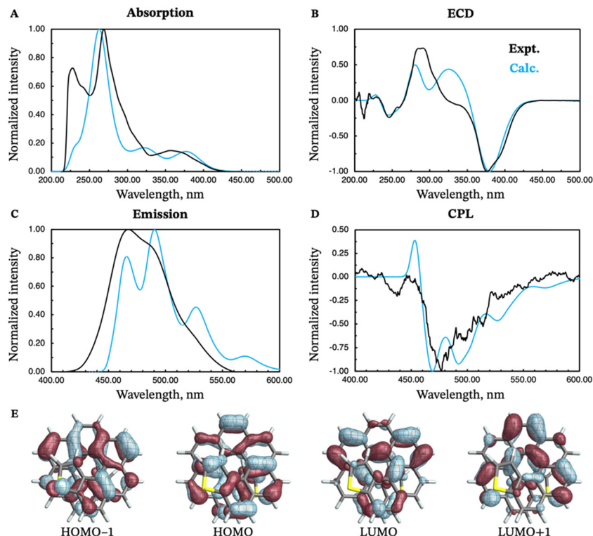
Fig. 5 Experimental (black curves) and calculated (blue curves) absorption (panel A), ECD (panel B), emission (panel C) and CPL (panel D) spectra of ( M )-exo-dithia[9]helicene 1 . Isosurfaces ( \pm 0.03 au) for the most relevant frontier molecular orbitals (HOMO-1, HOMO, LUMO, and LUMO+1) are shown in panel E. The calculated energies were shifted by -0.40 eV prior to conversion to wavelengths.
