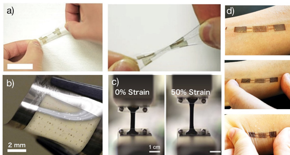
Fig. 2 Stretchable OECTs: (a) Optical images of a stretchable OECT. Adapted with permission from ref. 22 copyright 2019 Wiley-VCH; (b) stretchable OECT microelectrode arrays ( 10 \times 10 ) with channel length down to 5 \mu\text{m} . Adapted with permission from ref. 14 copyright 2017 American Chemical Society; (c) strain test of the stretchable system. Adapted with permission from ref. 32 copyright 2019 Wiley-VCH; (d) stretchable OECT e-skin. Adapted with permission from ref. 33 copyright 2019 Wiley-VCH.
