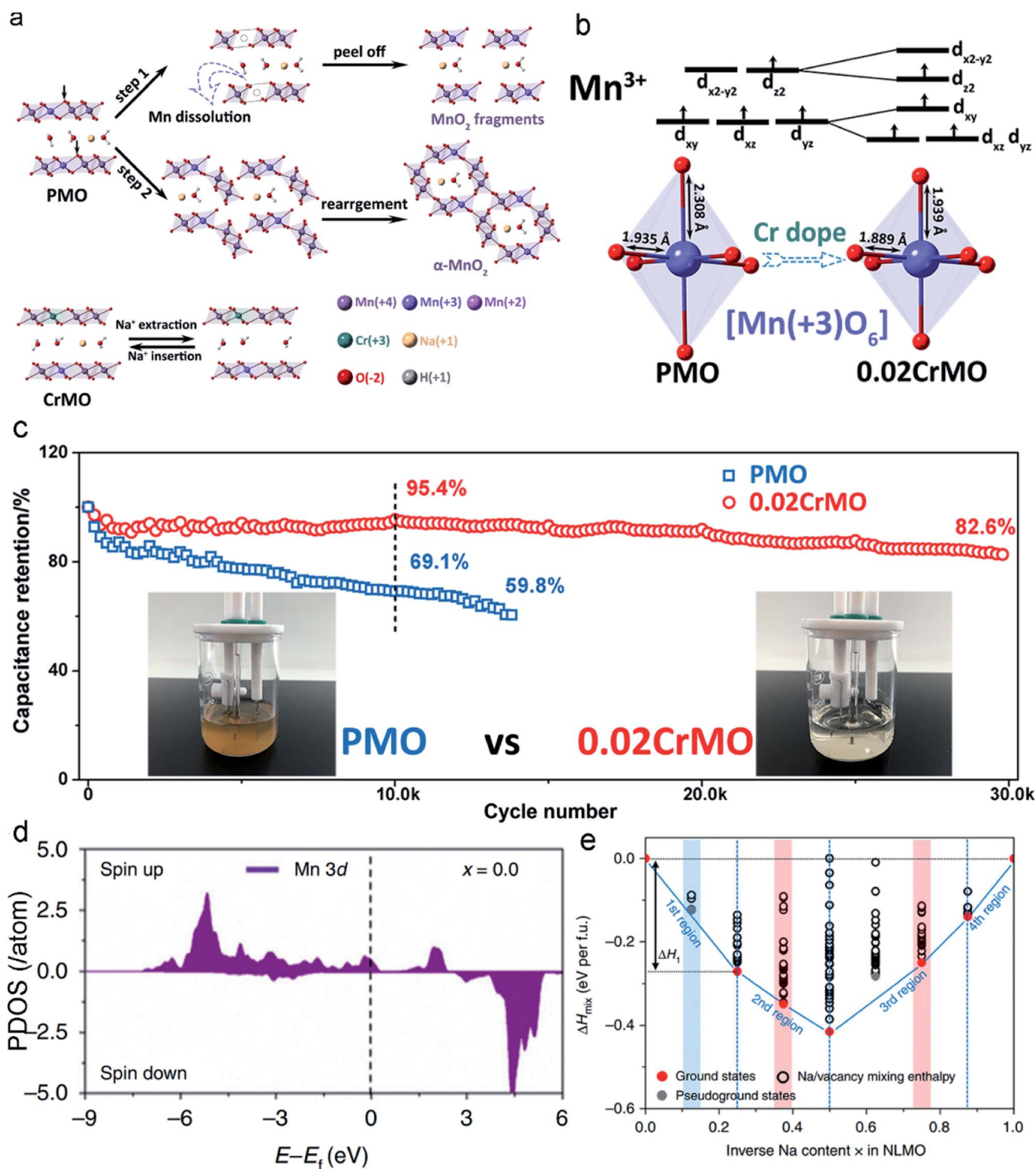
Fig. 8 (a) Mechanisms of Cr-doping for the stabilities of the \delta -MnO 2 . (b) The shortened Mn–O bonds after Cr-doping. (c) Cycling performances of the pristine \delta -MnO 2 and Cr-doped \delta -MnO 2 electrodes at a current density of 10 A g -1 . Reproduced with permission. 124 Copyright 2020 Royal Society of Chemistry. (d) The PDOS of the Mn 3+ sites in the layered Zn-doping Na[Li 0.25 Mn 0.75 ]O 2 . (e) The two atomic models include 8 Na atoms in each unit cell. Reproduced with permission. 34 Copyright 2019 Springer Nature.
