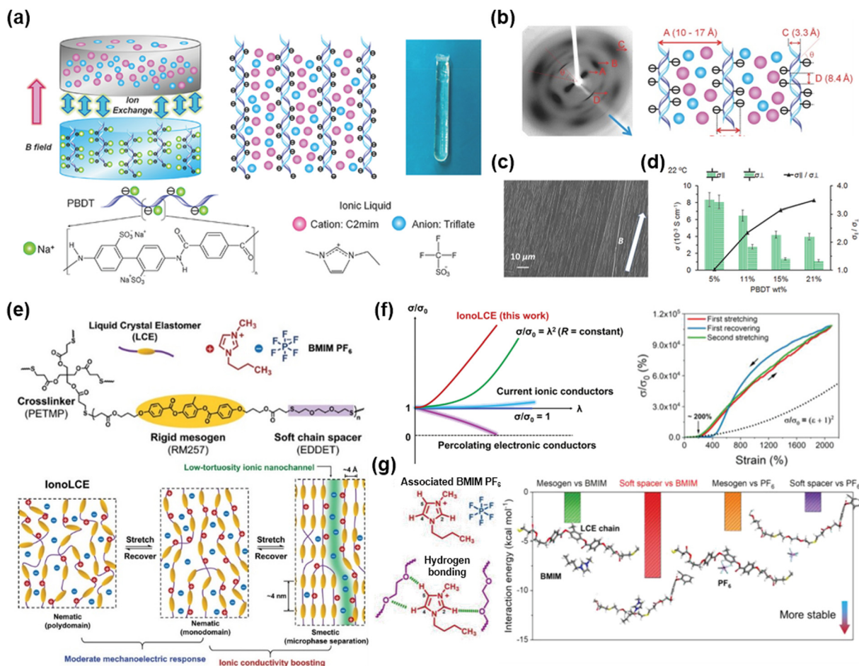
Fig. 13 Aligned iontronics based on liquid crystal elastomer (LCE)-IL composites. (a) A magnetically aligned PBDT-IL gel. (b) X-ray diffraction image of the gel and its corresponding diagram. (c) SEM image of the side-on surface of the gel. (d) Anisotropic ionic conductivity of the gel. Reproduced with permission from ref. 136. Copyright 2016, Wiley-VCH. (e) Molecular structures of the LonoLCE and schematics of stretch-induced ionic conductivity boost of the LonoLCE. (f) Mechanoelectric response of the LonoLCE and other ionic conductors. (g) Molecular interactions in the LonoLCE and calculated interaction energies. Reproduced with permission from ref. 137. Copyright 2021, Wiley-VCH.
