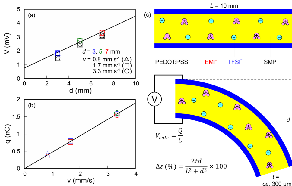
Fig. 8 Relation (a) between V and d and (b) between q and v of ionic SMP gel sensor ( W_{\text{IL}} = 25 \text{ wt\%} ) measured at d = 3 (blue), 5 (green), 7 \text{ mm} (red) and v = 0.8 ( \Delta ), 1.7 ( \square ), 3.3 \text{ mm s}^{-1} ( \circ ) with calculated voltages ( V_{\text{calc}} ) defined as V_{\text{calc}} = Q/C represented by black symbols where straight lines were obtained by fitting with the least-squares method. (c) Schematic illustration of a possible mechanism of piezoionic effect in ionic SMP gel sensor.
