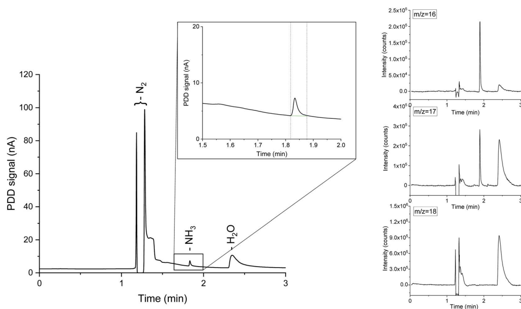
Fig. 1 On the left, the full chromatograph corresponding to 13.8 ppm of NH 3 in nitrogen. Ammonia is eluted at 1.83 minutes, while water appears at about 2.30 minutes. The enclosure highlights the region of the chromatograph around the ammonia elution time. On the right, the MS signal corresponding to the m/z 18, 17 and 16. At the ammonia retention time m/z 17 and 16 are the only contributions, demonstrating the absence of water interference.
