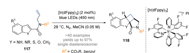
Scheme 34 Dearomative photoredox catalysed intramolecular [2 + 2] cycloaddition of indoles. 40
