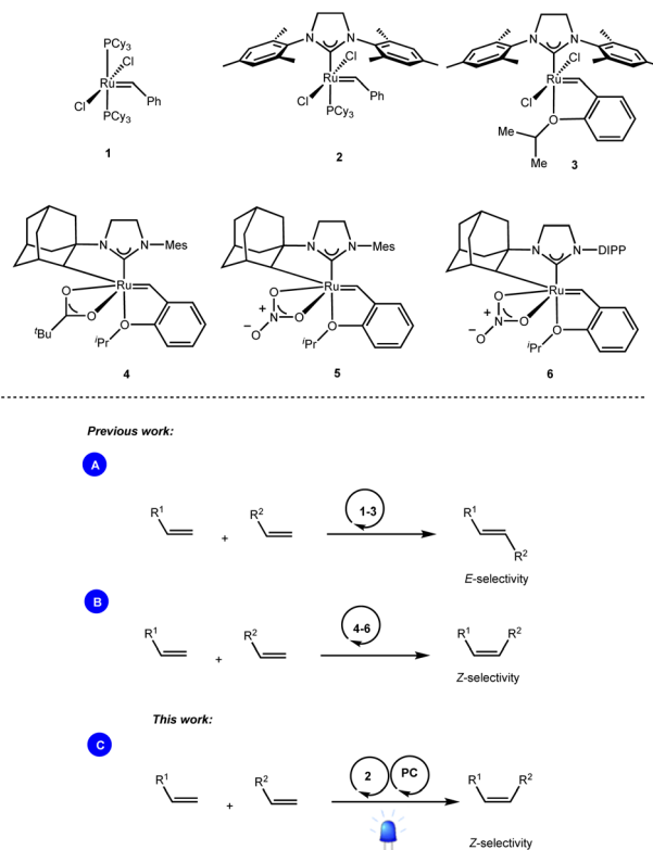
Scheme 1 Ru-based catalysts enabling stereoselective olefin cross-metathesis reactions.
