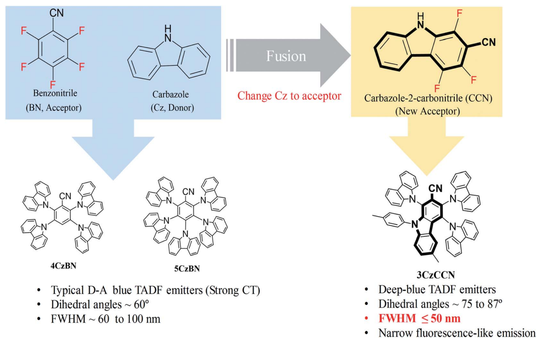
Scheme 1 New acceptor (CCN) by fusing carbazole and benzonitrile for narrow CT emissions of deep-blue D–A type TADF emitters.
