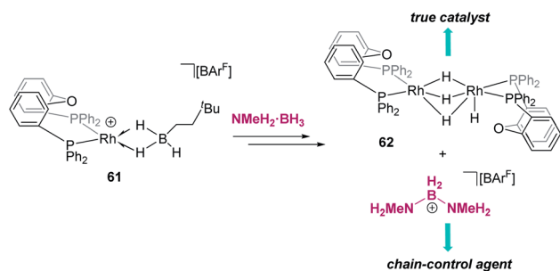
Scheme 63 Dehydropolymerization of \text{NMe}_2\text{H}\cdot\text{BH}_3 mediated by 61 .
