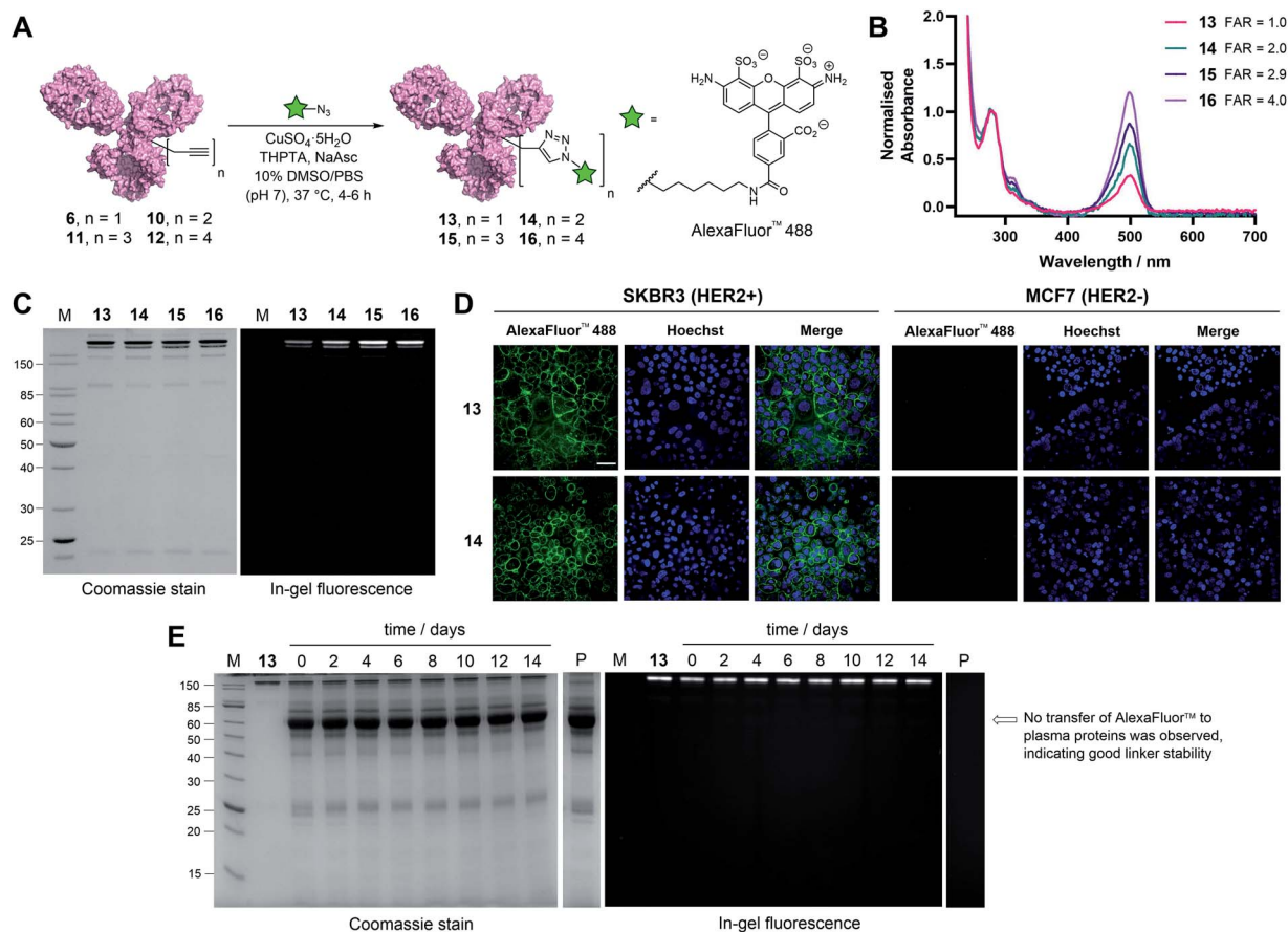
Fig. 4 Functional modification and stability analysis of TetraDVP-modified trastuzumab. (A) Reaction of TetraDVP conjugates 6 , 10 , 11 and 12 with AlexaFluor ™ 488 azide to form fluorescent conjugates 13 , 14 , 15 and 16 . PBS = phosphate-buffered saline. (B) UV/vis spectra of conjugates 13 , 14 , 15 and 16 . Absorbance was normalised at 280 nm. Absorbance at 495 nm was used to calculate the fluorophore-to-antibody ratio (FAR). (C) Analysis of conjugates 13 , 14 , 15 and 16 by SDS-PAGE under reducing conditions; M = molecular weight marker. Left gel is after Coomassie staining, right gel is in-gel fluorescence measured before staining. (D) Live cell microscopy images of HER2-positive SKBR3 cells and HER2-negative MCF7 cells after treatment with 13 or 14 shows selective labelling of antigen-positive cells. Scale bar represents 50 μm. (E) Stability analysis of conjugate 13 in human plasma by SDS-PAGE; M = molecular weight marker, P = human plasma, days of incubation are depicted above the representative lane. Left gel is after Coomassie staining, right gel is in-gel fluorescence measured before staining. No transfer of AlexaFluor ™ 488 to human serum albumin (66.5 kDa, indicated by the arrow) or any other plasma proteins is observed over the 14 day incubation period.
