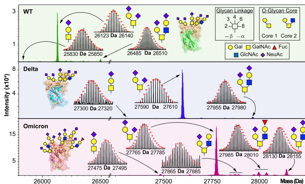
Fig. 3 O-glycoform characterization of the S-RBD variants. Deconvoluted MS of the S-RBD proteoforms are shown with all major O-glycan assignments for the WT (green), Delta (blue), and Omicron (pink) variants. Insets show the isotopically and baseline resolved S-RBD proteoform MS spectra allowing for accurate determination of individual intact glycoforms. MS data were collected on the 12 T FTICR-MS. All individual ion assignments are within 1 ppm from the theoretical mass and theoretical isotopic distributions are indicated by the red dots. Assignments of the glycan structures are marked in the spectrum with the legend shown as an inset. PDB: 6M0J, 7WBQ, 7WBP.
