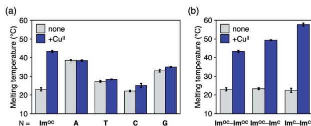
Fig. 5 Melting temperatures of duplexes containing an \text{Im}^{\text{OC}}\text{-N} base pair (1·2N; N = \text{A}, \text{T}, \text{C}, \text{G} ) in the absence and presence of 1 equiv. of \text{Cu}^{\text{II}} . (b) Melting temperatures of duplexes containing an \text{Im}^{\text{OC}}\text{-Im}^{\text{OC}} (1·2), an \text{Im}^{\text{OC}}\text{-Im}^{\text{C}} (1·8), or an \text{Im}^{\text{C}}\text{-Im}^{\text{C}} base pair (7·8) in the absence and presence of 1 equiv. of \text{Cu}^{\text{II}} . [duplex] = 2.0 \mu\text{M} and [\text{Cu}^{\text{II}}]/[\text{duplex}] = 0 or 1 in 10 mM HEPES buffer (pH 7.0) and 100 mM \text{NaCl} . N = 3 . The error bars represent the standard errors.
