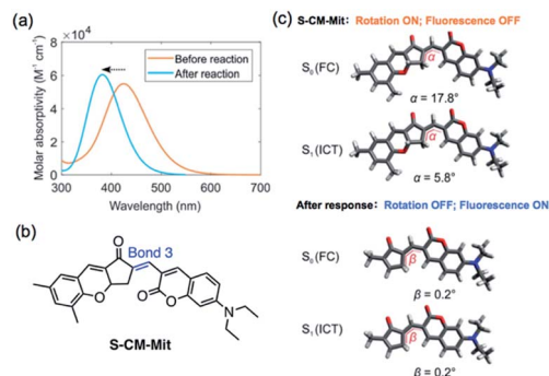
Fig. 4 (a) Calculated UV-vis absorption spectra of CM-Mit and the product after the reaction of CM-Mit and thiol. (b) The simplified structure of CM-Mit ( S-CM-Mit ). (c) S-CM-Mit and the product after the response in the ground state (the Franck–Condon state) and the ICT state. The insets show the dihedral angles ( \alpha and \beta ) along with bond 3.
