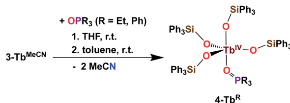
Scheme 6 Synthesis of 4-Tb R (R = Et, Ph). 5c
