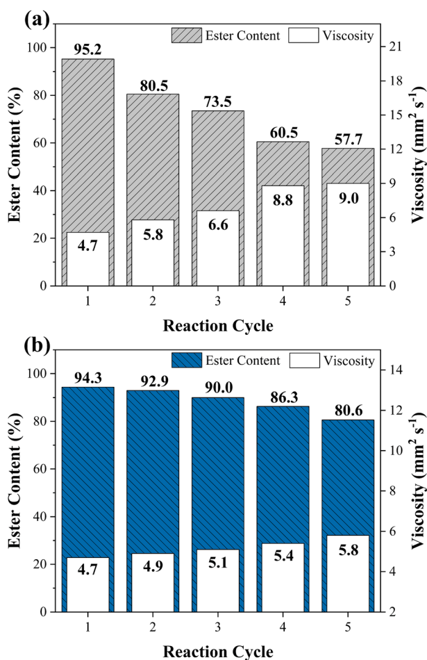
Fig. 10 Reuse study of \text{WO}_3/\text{CuFe}_2\text{O}_4 magnetic catalyst in the transesterification reaction (a) with heat treatment and (b) without heat treatment at 500 °C/3 h.
