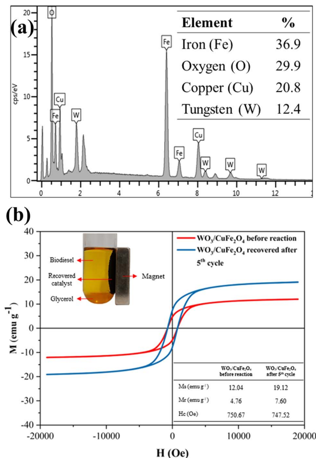
Fig. 11 Analysis of (a) EDS and (b) VSM of the \text{WO}_3/\text{CuFe}_2\text{O}_4 catalyst recovered after the 5th reaction cycle.
