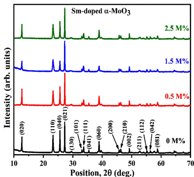
Fig. 2 XRD patterns of pristine and Sm-incorporated \alpha - \text{MoO}_3 nanoparticles.
