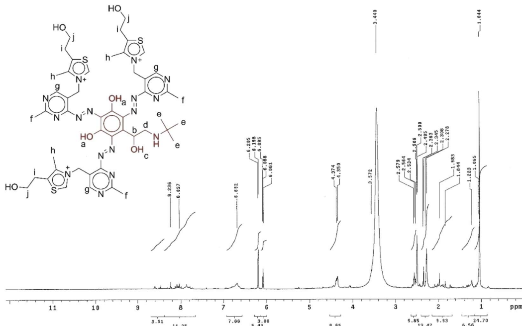
Fig. 3 1 H-NMR spectrum of the thiamine-TBDA azo dye in deuterated DMSO.
