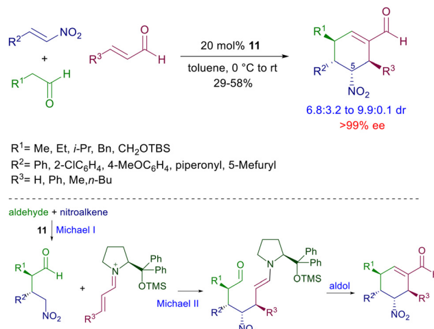
Scheme 16 Three-component coupling involving a cascade Michael-Michael-aldol condensation catalyzed by 11 .
