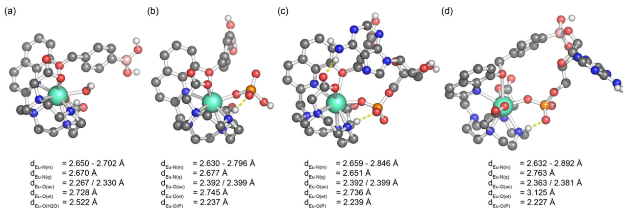
Fig. 7 Molecular geometries of [\text{Eu}\cdot\text{pBOH}_2]^+ bound to (a) water, (b) hydrogen phosphate, (c) AMP bound in a monodentate manner and (d) AMP bound in a cyclic manner involving a boronate ester-ribose interaction. Bond distances of Eu(III) to donor atoms are shown: N(m) – macrocycle, N(q) – quinoline, O(ac) – acetate, O(et) – ether, O(H 2 O) – water, O(P) – phosphate.
