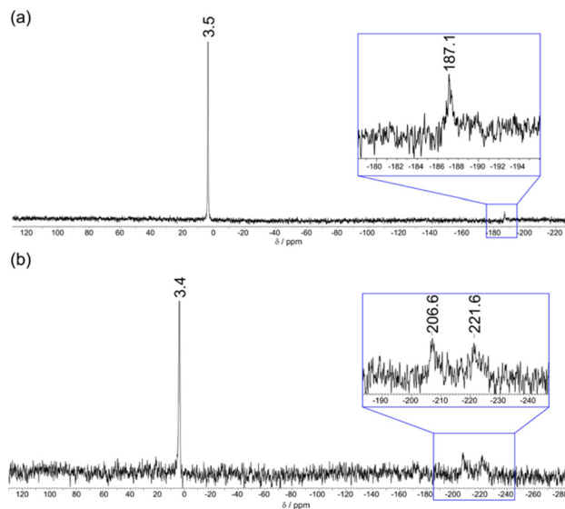
Fig. 6 ^{31}\text{P} NMR spectra (202.5 MHz, \text{D}_2\text{O} , pD 7.4) of (a) [\text{Eu}\cdot\text{pBOH}_2]^+ (1 mM) with phosphate (10 mM) showing ^{31}\text{P} signals for both bound and unbound phosphate; (b) [\text{Eu}\cdot\text{pBOH}_2]^+ (1 mM) with AMP (1 mM) showing a sharp ^{31}\text{P} signal for unbound AMP and two broad signals indicating exchange between two binding modes for AMP.
