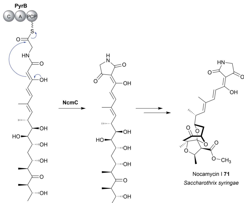
Fig. 32 Chain release catalysed by standalone Dieckmann cyclases. (A) In pyrroindomycin ( 70 ) biosynthesis chain release is catalysed via a Dieckmann condensation. Two enzymes, PyrE3 and PyrE4, are both capable of catalysing this reaction. (B) Formation of the tetramate ring in nocamycin I ( 71 ) is catalysed by the \alpha/\beta hydrolase NcmC.
