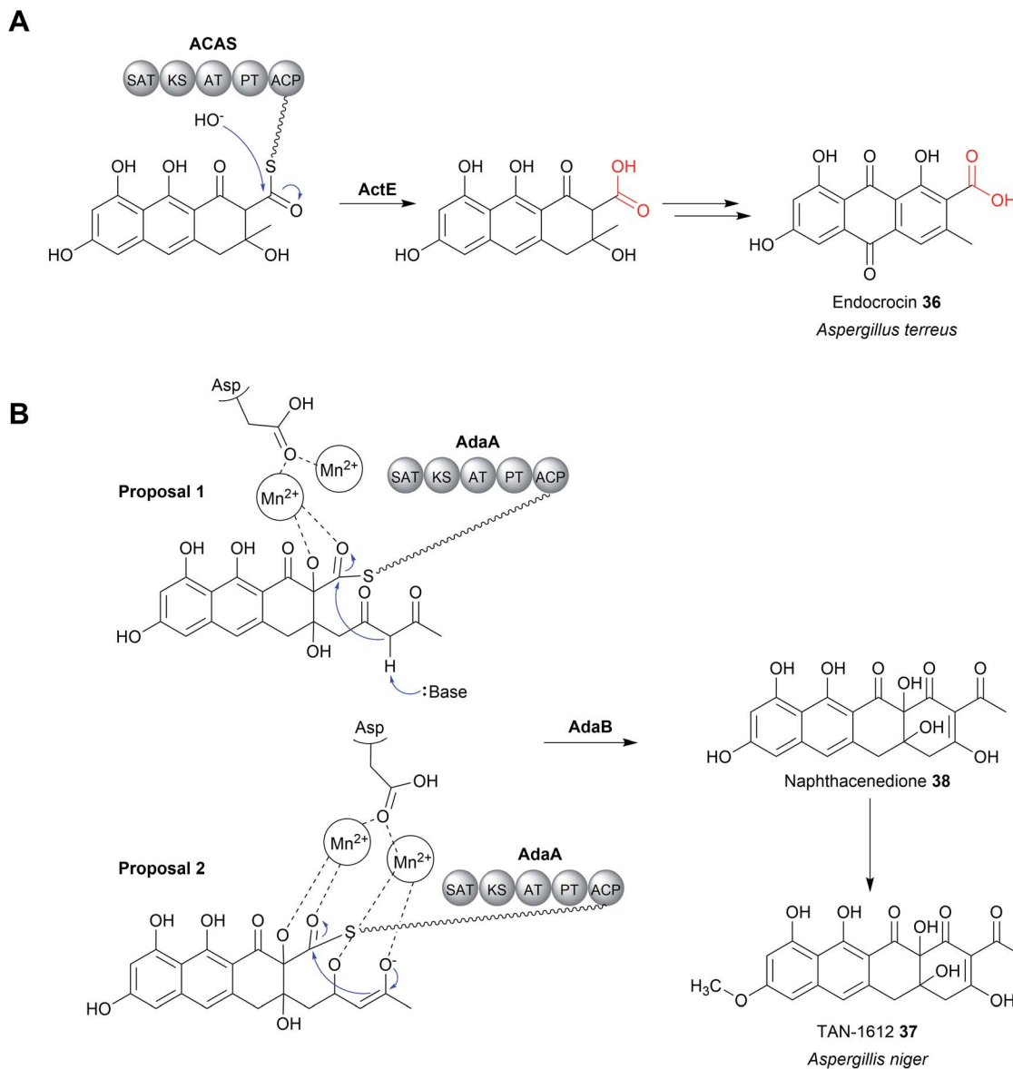
Fig. 15 Chain release catalysed by metallo- \beta -lactamase (MBL) thioesterase. (A) The MBL ActE is responsible for chain release of the endocrocin precursor from the PKS ACAS. (B) The two possible mechanisms have been proposed for the \text{Mn}^{2+} dependent Dieckmann condensation catalysed by AptB/AdaB.
