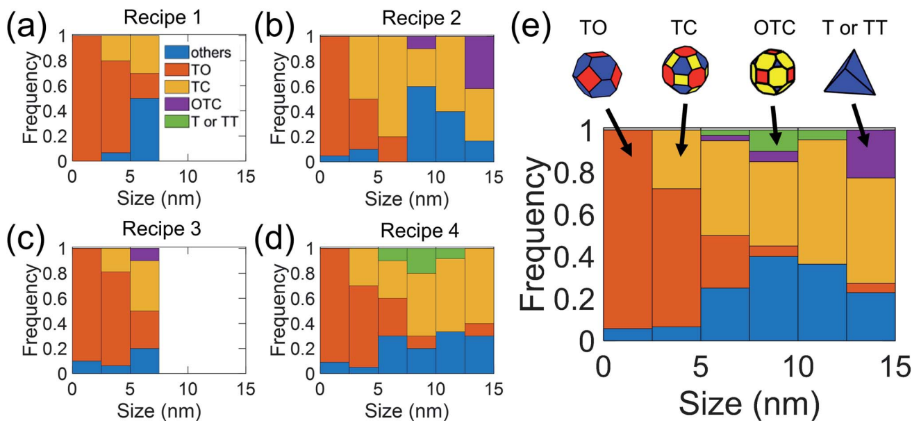
Fig. 3 The distribution of particle shapes is size dependent. Histograms show the frequency of different nanoparticle shapes within each size range. The colors correspond to particle shapes as defined in the legend in panel (a), using the following acronyms: truncated octahedron (TO), truncated cuboctahedron (TC), over-truncated cuboctahedron (OTC), and tetrahedron or truncated tetrahedron (T or TT). Results are shown for each of the four synthesis recipes (WI at low (a) and high (b) temperatures; and SEA at low (c) and high (d) temperatures). Panel (e) contains the combined results from all synthesis recipes. Inset above the figure are schematics of the four particle shapes.
