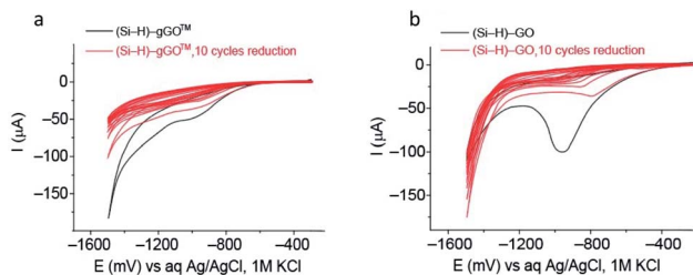
Fig. 6 Electrochemical reduction of gGO and GO (Hummers' method). Ten consecutive cyclic voltammograms for the electrochemical reduction of (a) Si-gGO and (b) Si-GO (Hummers' method) in 0.1 M phosphate buffer solution at pH 7.4, and a scan rate of 50 mV s -1 . The potential is presented in mV vs. Ag/AgCl, 1 M KCl. The reduction wave is centred around -950 mV for both carbon-2D materials. In both systems, the charge decreases by 80–90% after 10 cycles.
