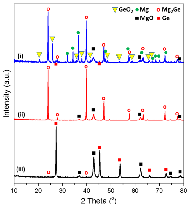
Fig. 1 PXD patterns of samples: (i) after the 1st MW irradiation of 20 s, (ii) after the 2nd MW irradiation of 60 s, and (iii) after thermal dealloying (in air) at 550^\circ\text{C} for 11 h. (See synthesis steps in Scheme 1, for reference.).
