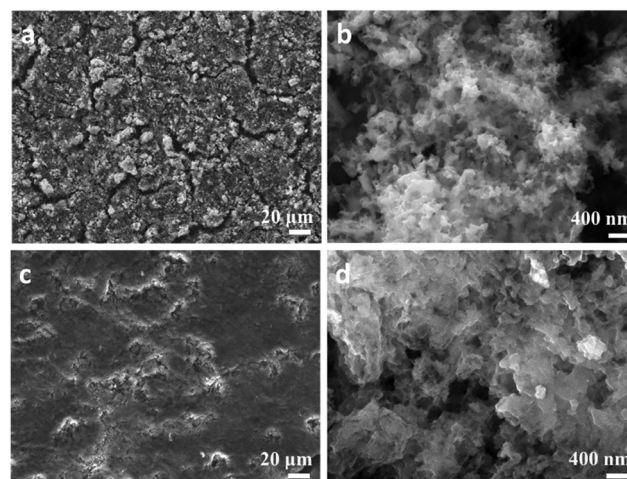
Fig. 4 SEM images of NP Ge electrodes, (a), (b) before cycling; and (c), (d) after cycling tests at 1.0 \text{ A g}^{-1} for 200 cycles.
