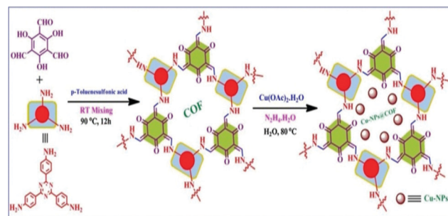
Scheme 32 The synthesis of Cu-NPs@COF. Reproduced with permission from ref. 58; copyright: 2020, Journal of CO 2 Utilization.
