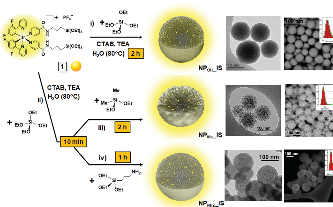
Scheme 1 Schematic representation of the synthesis of in situ hybrid mesoporous organometallo-silica nanoparticles ( NP OH-IS , NP Me-IS and NP NH 2 -IS ), including TEM and SEM images of each, showing their textural differences, as well as their DLS size distributions.
