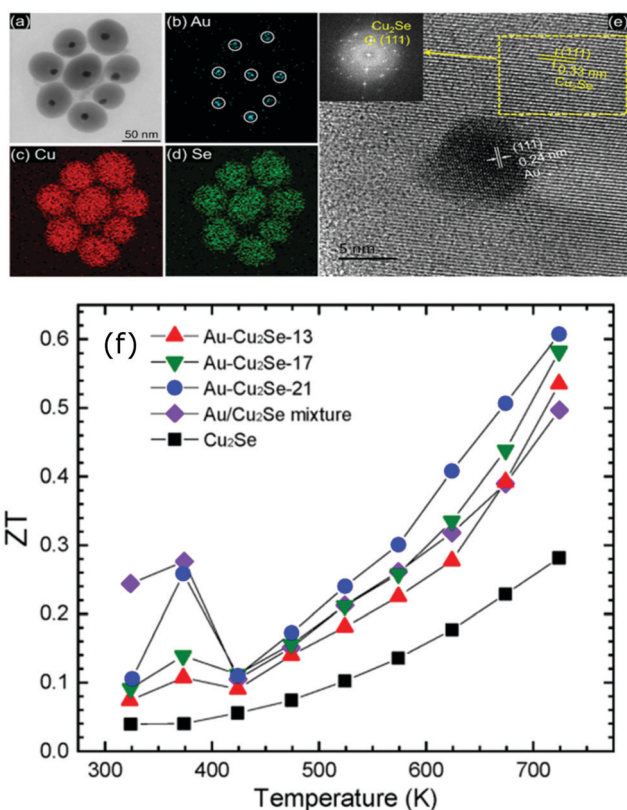
Fig. 8 (a) Transmission electron microscopes (TEM) images of \text{Au}@ \text{Cu}_2\text{Se} nanoparticles and the elemental mapping pictures of (b) Au, (c) Cu, (d) Se, (e) shows the high resolution-TEM images of a \text{Au}@ \text{Cu}_2\text{Se} nanoparticles (inset is the corresponding Fourier transform), and (f) shows the figure of merit ( zT ) of \text{Au}@ \text{Cu}_2\text{Se} core-shell nanocomposite samples of different shell thicknesses (21, 17, and 13 nm) along with pure \text{Cu}_2\text{Se} , \text{Au}/\text{Cu}_2\text{Se} mixture sample. Reproduced with permission from ref. 111, Copyright 2020 American Chemical Society.
