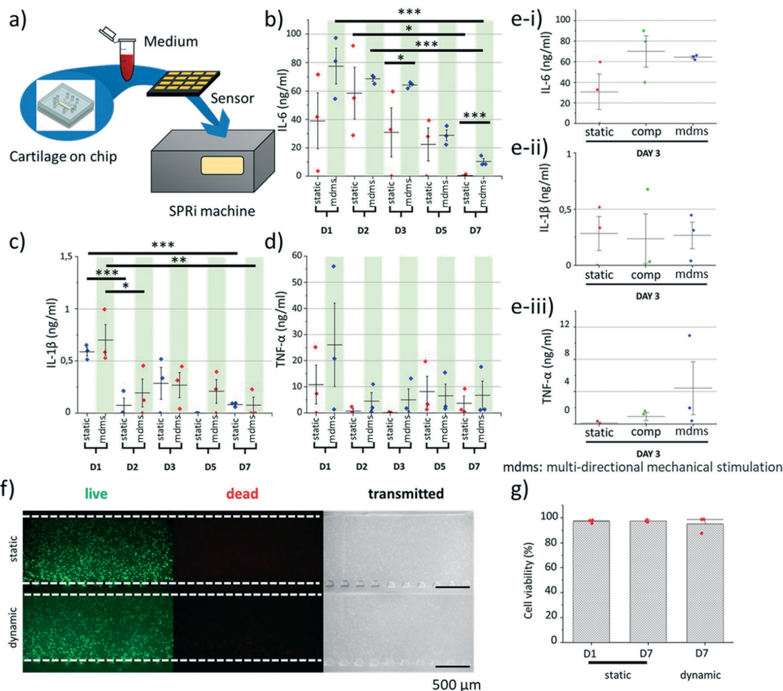
Fig. 3 Cytokine release in the cartilage-on-chip device as a function of time analyzed by SPRi. a) Medium is collected from the devices, diluted before off-line analysis by SPRi. Quantification of the secretion of IL-6 (b), IL-1β (c), and TNF-α (d) in the medium for static culture (red dots) and multi-directional mechanical stimulation (mdms) (blue dots) on different days for 3 independent samples (1 sample = 3 devices). e) Comparison of static culture (red), compression only (green) and multi-directional mechanical stimulation (mdms) at day 3 for IL-6 (i), IL-1β (ii) and TNF-α (iii). f) Cell viability assay using calcein AM (green-live) and ethidium homodimer (red-dead); fluorescence microscopy and corresponding bright-field microscopy images for static and compression only culture. g) Quantification of the viability of human chondrocytes in static (day 1 & 7) and dynamic (compression only, day 7) culture. Scale bar = 500 μm. P_{\text{value}}: 0.1 > P_{\text{value}} > 0.05^* , 0.05 > P_{\text{value}} > 0.01^{**} , 0.01 > P_{\text{value}} > 0.001^{***} .
