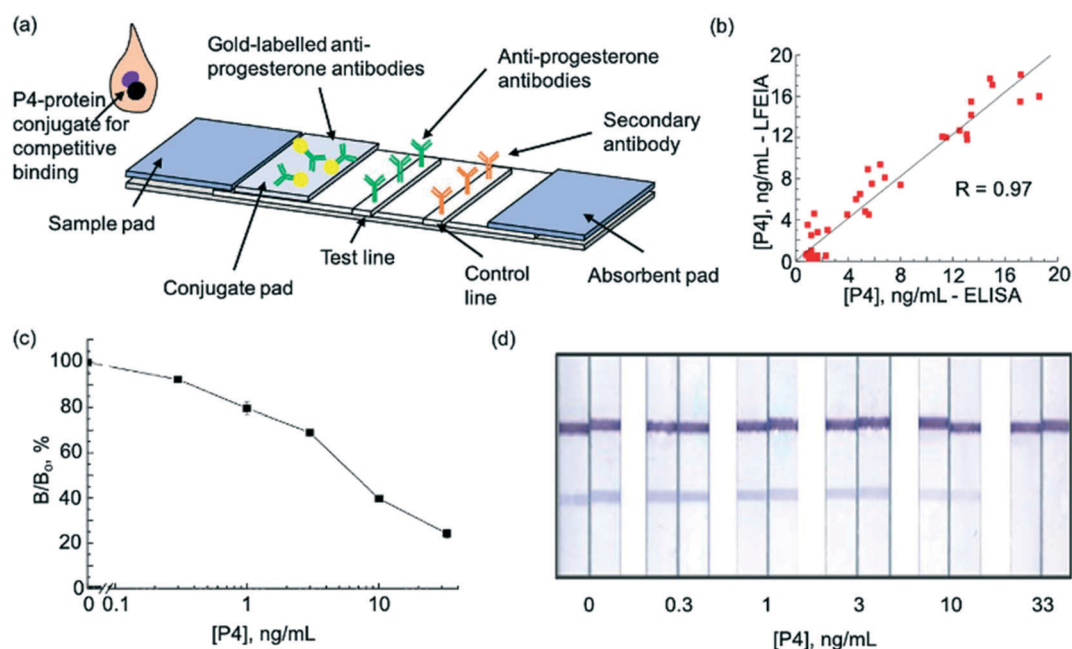
Fig. 3 Enzyme lateral flow immunoassay for pregnancy testing in cows. (a) Schematic illustration of test strip (b) comparison of P4 measurements in cows' milk using ELISA and LFEIA (c) P4 LFA calibration curve. (d) Visualisation of calibration curve after staining. Reproduced with permission. 57,78 Copyright 2015, Elsevier.
