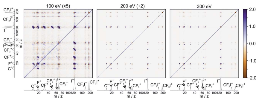
Fig. 5 ToF-ToF covariance maps obtained following electron ionisation of \text{CF}_3\text{I} at electron energies of 100, 200, and 300 eV. Saturated ToF-ToF covariance maps for the 200 and 300 eV data, in which weaker covariance signals are visible, can be found in the ESI.†
