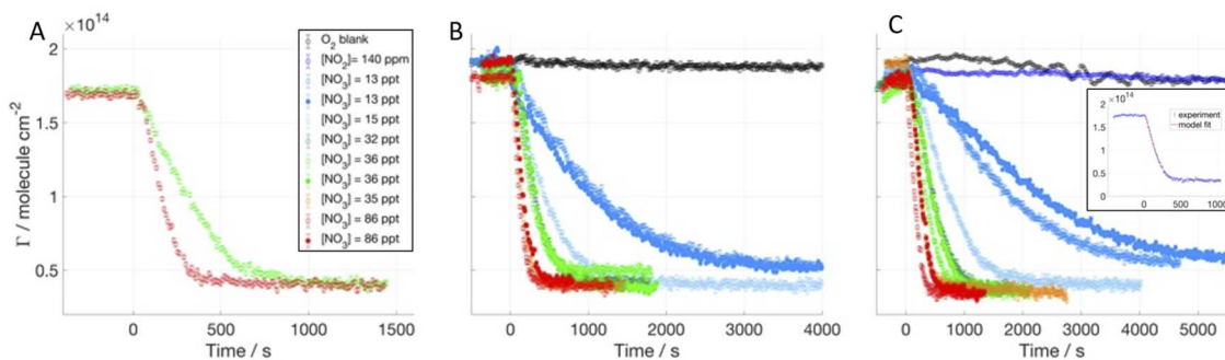
Fig. 2 Surface excess decays of dOAhOA (A), dOAhSA (B) and dOAhMO (C) exposed to different [\text{NO}_3] ; mean values of \text{NO}_3 mixing ratios are displayed in the legend (1 ppt = 2.7 \times 10^7 molecule per \text{cm}^3 ), \text{NO}_3 is admitted at t = 0 s. In the insert, data and fit are shown for dOAhMO exposed to [\text{NO}_3] = 86 ppt.
