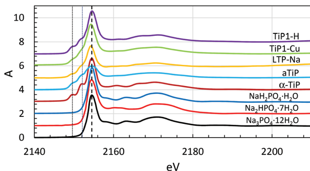
Fig. 4 Normalised phosphorus K edge XANES absorption edges of solid titanium(IV) and sodium phosphates. Offset steps: 1.0. The help lines are at 2149.6 and 2152.1 eV; sample 1 – TiP1-H , sample 2 – \alpha-TiP , sample 4 – aTiP , sample 5 – LTP-Na , sample 8 – TiP1-Cu (no data were collected on samples 3, 6, 7, 9 and 10).
