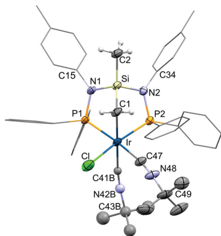
Fig. 6 ORTEP plot of [\text{IrCl}(\kappa^3\text{C},\text{P},\text{P}'\text{-(SiNP-H)})(\text{CN}^t\text{Bu})_2]^+ ( 4^+ ). For clarity, most hydrogen are omitted and the tolyl and phenyl rings are represented in a wireframe style. Selected bond lengths (Å) and angles ( ^\circ ) are given in ESI.†
