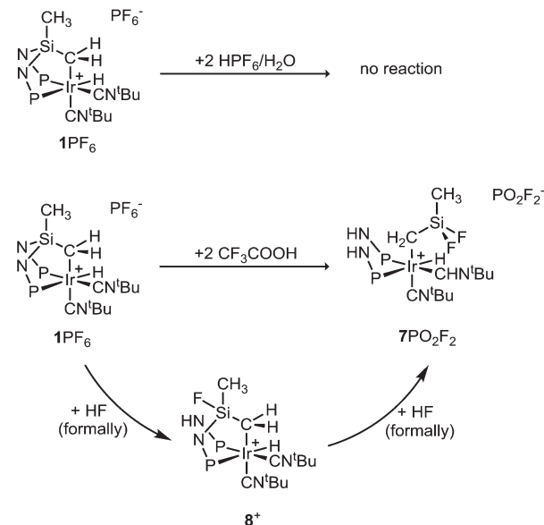
Scheme 6 Reaction of [\text{IrH}(\kappa^3\text{C},P,P'-\text{SiNP-H})](\text{CN}^t\text{Bu})_2[\text{PF}_6] with \text{HPF}_6 or \text{CF}_3\text{COOH} .
