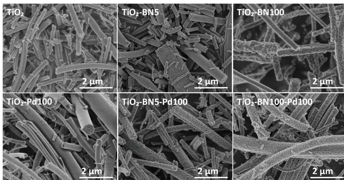
Fig. 2 SEM images of \text{TiO}_2 , \text{TiO}_2 -BN5, \text{TiO}_2 -BN100, \text{TiO}_2 -Pd100, \text{TiO}_2 -BN5-Pd100 and \text{TiO}_2 -BN100-Pd100 nanocomposites.
