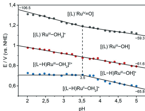
Fig. 5 Pourbaix diagram of [\text{Ru}(\text{tpy})(\text{pic-PO}_3\text{H}_2)(\text{H}_2\text{O})]^+(\text{Cl})^- immobilised on a meso -ITO electrode in the pH range of 2.0–5.0 ( \text{pK}_\text{a} value is denoted by the vertical dashed line, slopes are given in \text{mV pH}^{-1} ).
