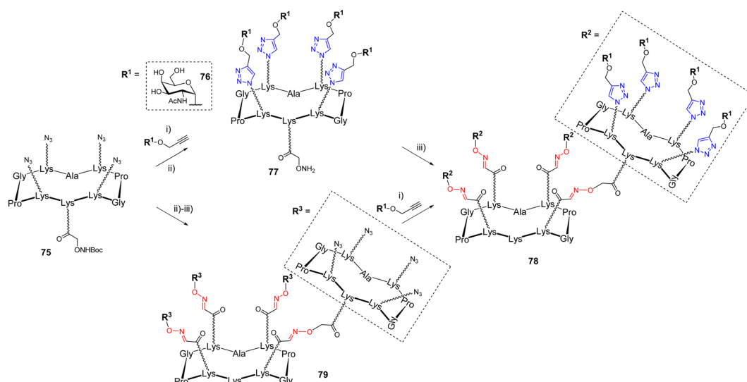
Scheme 15 Convergent synthesis of the hexadecavalent GalNAc glycodendrimer 78 by CuAAC/OL. Reagents and conditions: (i) \text{CuSO}_4 \cdot 5\text{H}_2\text{O} , THPTA, sodium ascorbate, DMF/PBS buffer (pH 7.5) (1 : 1), r.t., 2 h, 70% (divergent synthesis); (ii) TFA/ \text{H}_2\text{O} (6 : 4), r.t., 1 h, 77% over two steps for 77 ; (iii) 51 , 0.1% TFA in \text{H}_2\text{O} , 37 °C, 45 min, 90% for 78 ; 85% for 79 .
