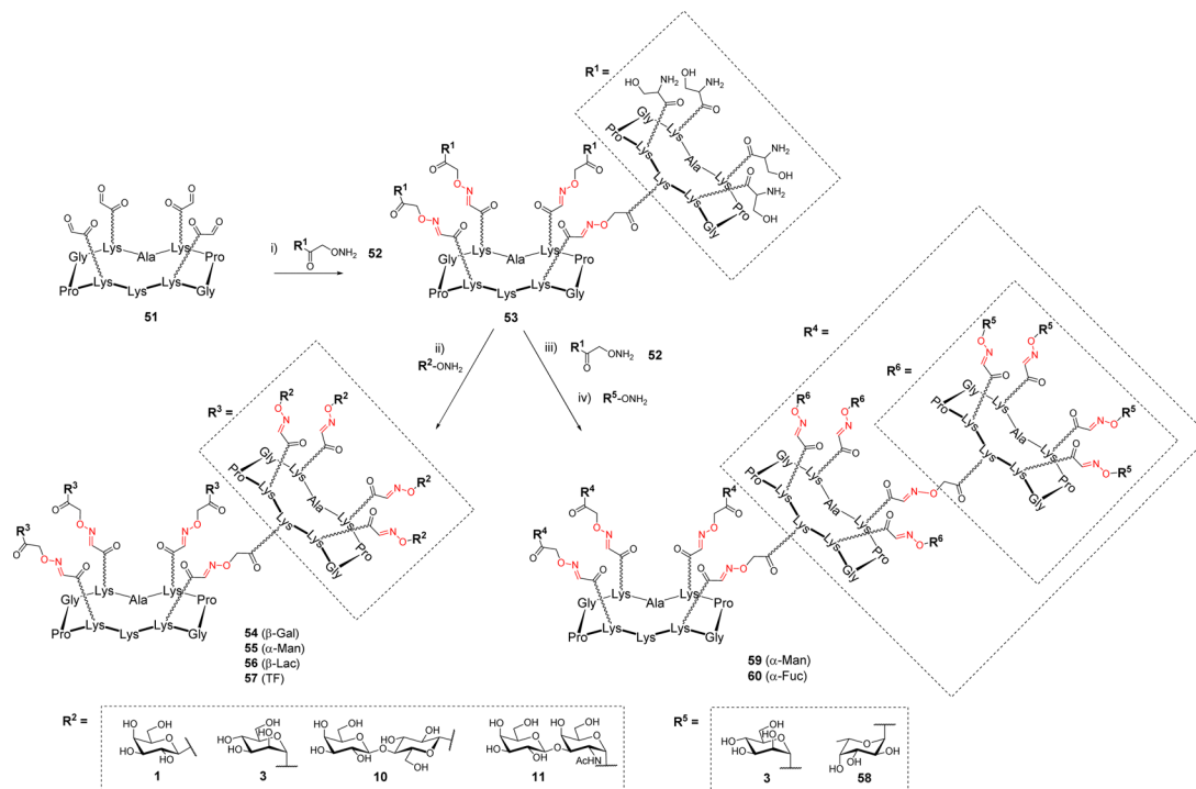
Scheme 11 Extension of the cyclopeptide valency from 16 to 64 by iterative oxime ligation. Reagents and conditions: (i) 0.1% TFA in \text{H}_2\text{O} , 37 °C, 4 h, acetone quenching; (ii) \text{NaIO}_4 , \text{H}_2\text{O} , r.t., 30 min then 0.1% TFA in \text{H}_2\text{O} , 37 °C, 4 h, 65–88%; (iii) 0.1% TFA in \text{H}_2\text{O} , 37 °C, 1 h, acetone quenching then \text{NaIO}_4 , \text{H}_2\text{O} , r.t., 30 min, 88%; (iv) 0.1% TFA in \text{H}_2\text{O} , 37 °C, 4 h, 83–85%.
