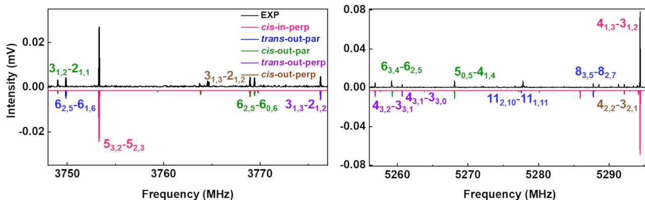
Fig. 3 Parts of the 2–8 GHz rotational spectrum of AMPA with the labelling scheme of the rotational transitions as J'_{K'_a}K'_c \leftarrow J''_{K''_a}K''_c . The top part shows the experimental spectrum and the bottom part represents the simulations using the fitted rotational parameters for AMPA conformers (Table 2). The relative intensities are based on the predicted dipole moment components (Table 1).
